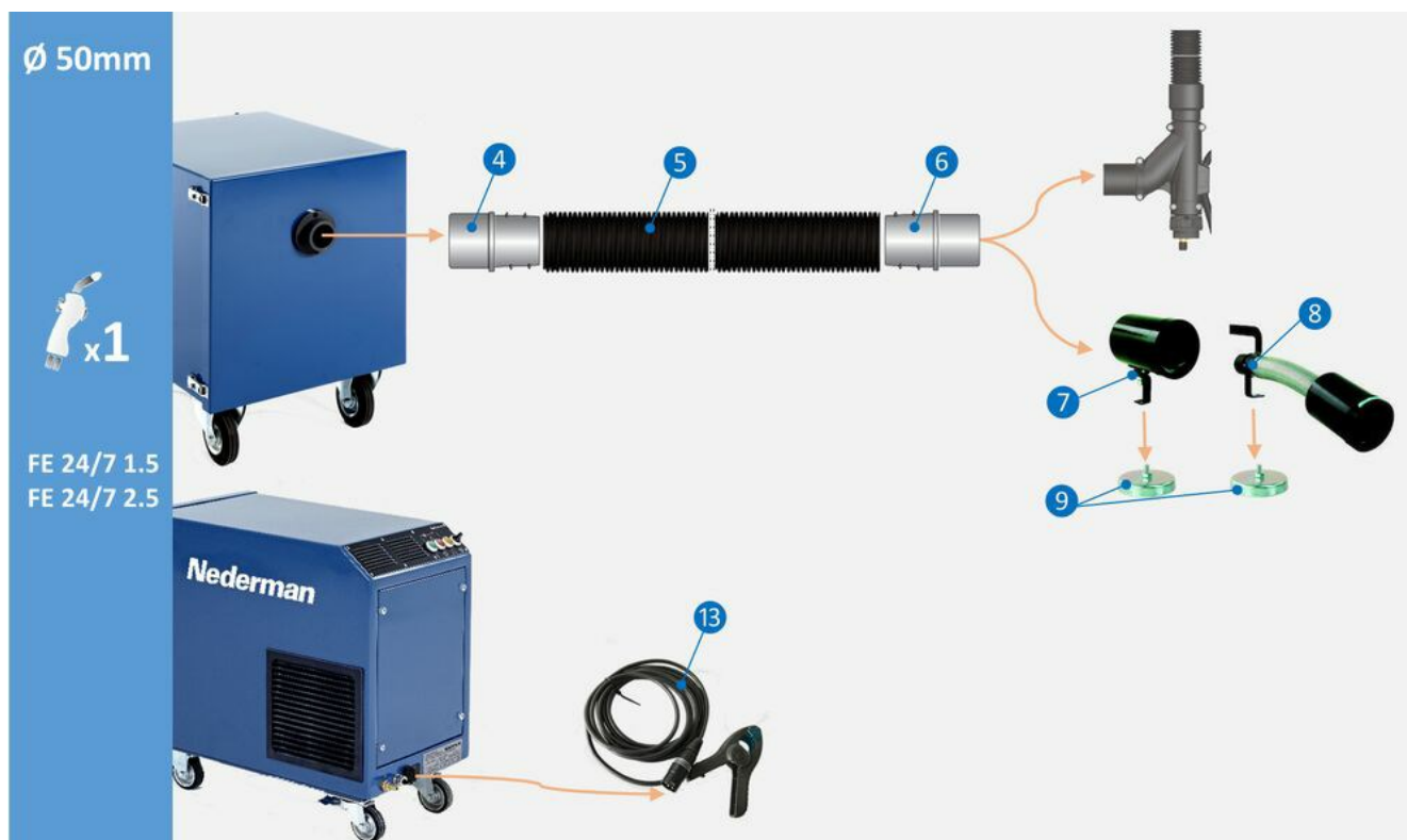
Accessories configuration for one user, 50mm welding machine connection. (4) Hose Coupler M50-50P, art.no. 55999416 (5) Hose PE-51 L=5m, art.no. 55999412 (6) Hose Coupler F50-50P, art.no. 55999417 (7) Nozzle CWN-S 105/50 Silencer, art.no. 55999415 (8) Nozzle CWN-S 105/50L Silencer, art.no. 55999414 (9) Magnetic foot for nozzle CWN-S, art.no. 55999419 (13) Sensor Clamp with plug for automatic start/stop, art.no. 55999410
